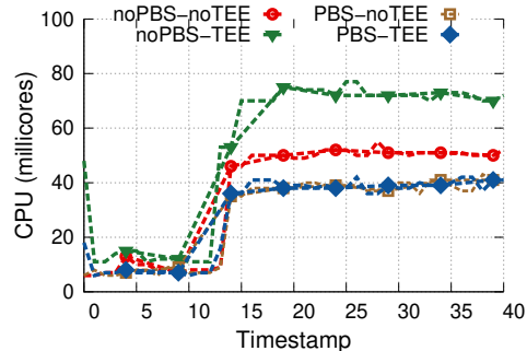
CPU usage: op-geth (30 TPS)
