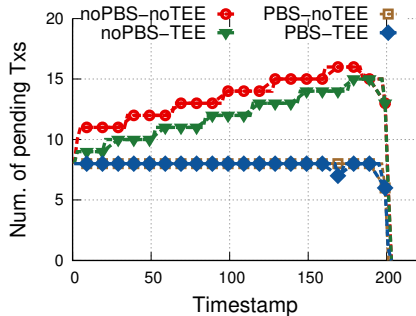
Pending Tx
