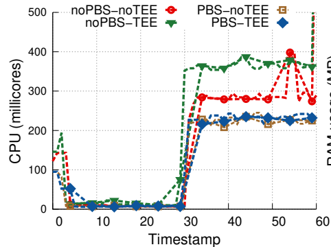
CPU usage (op-geth)
