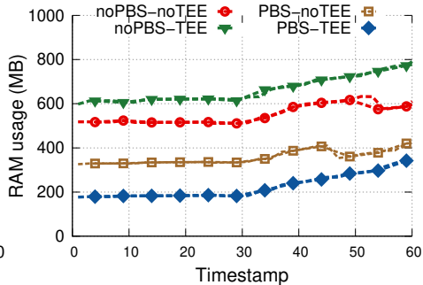
RAM usage: op-geht (270 TPS)
