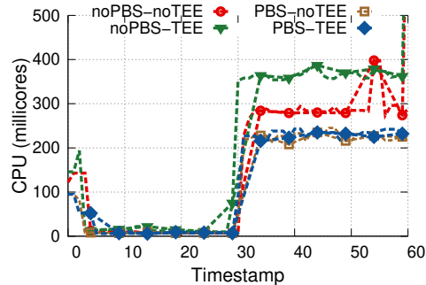
CPU usage: op-geht (270 TPS)
