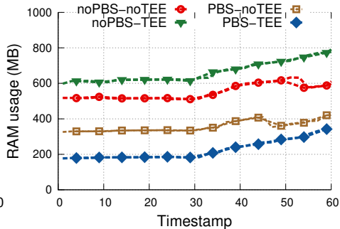
RAM usage: op-geth (270 TPS)
