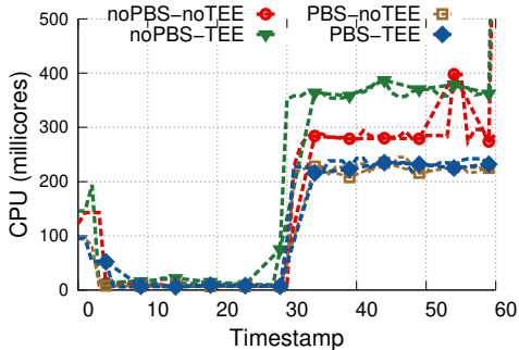
CPU usage: op-geth (270 TPS)
