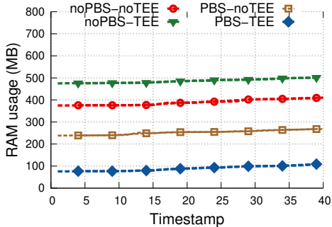
RAM usage: op-geth (270 TPS)
