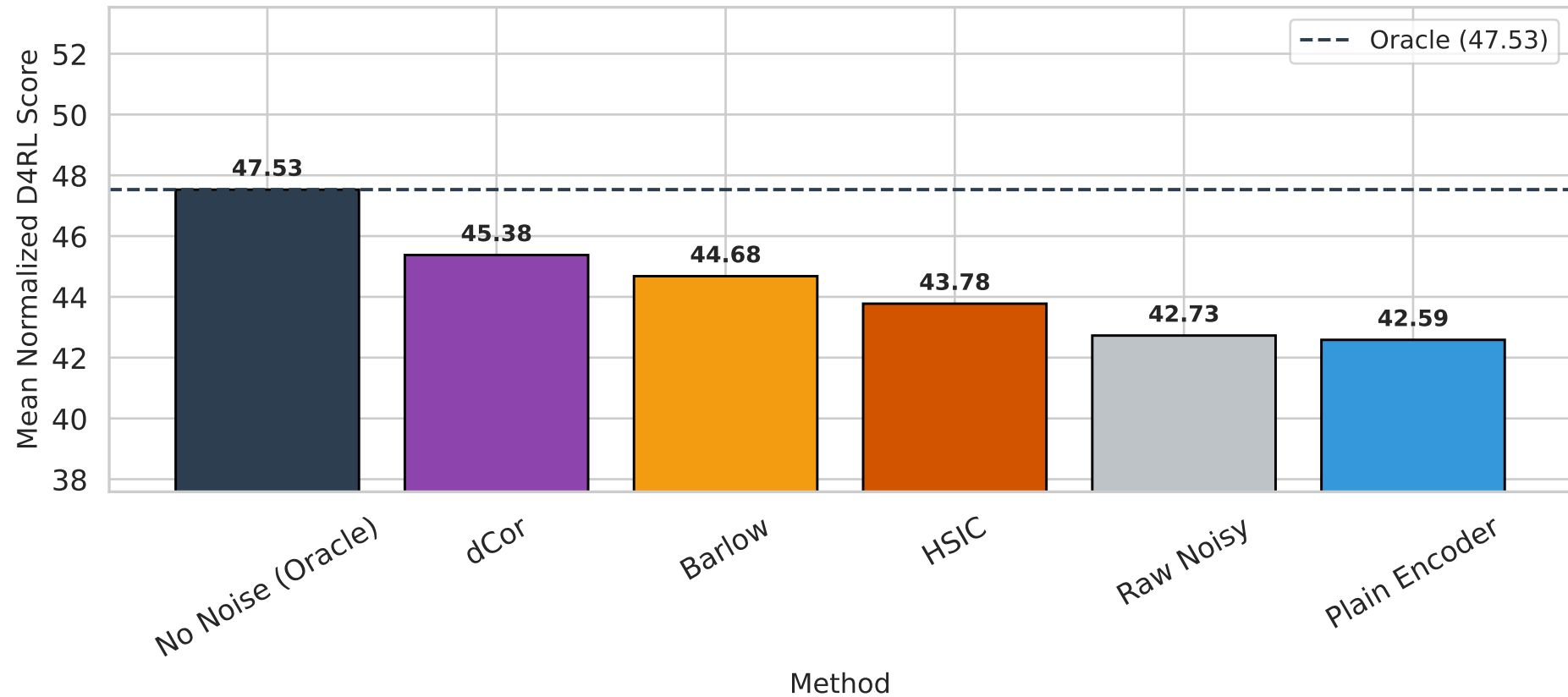
Step 1 — Global Mean Normalized Score (Nonlinear Noise, All 16 Configs)
