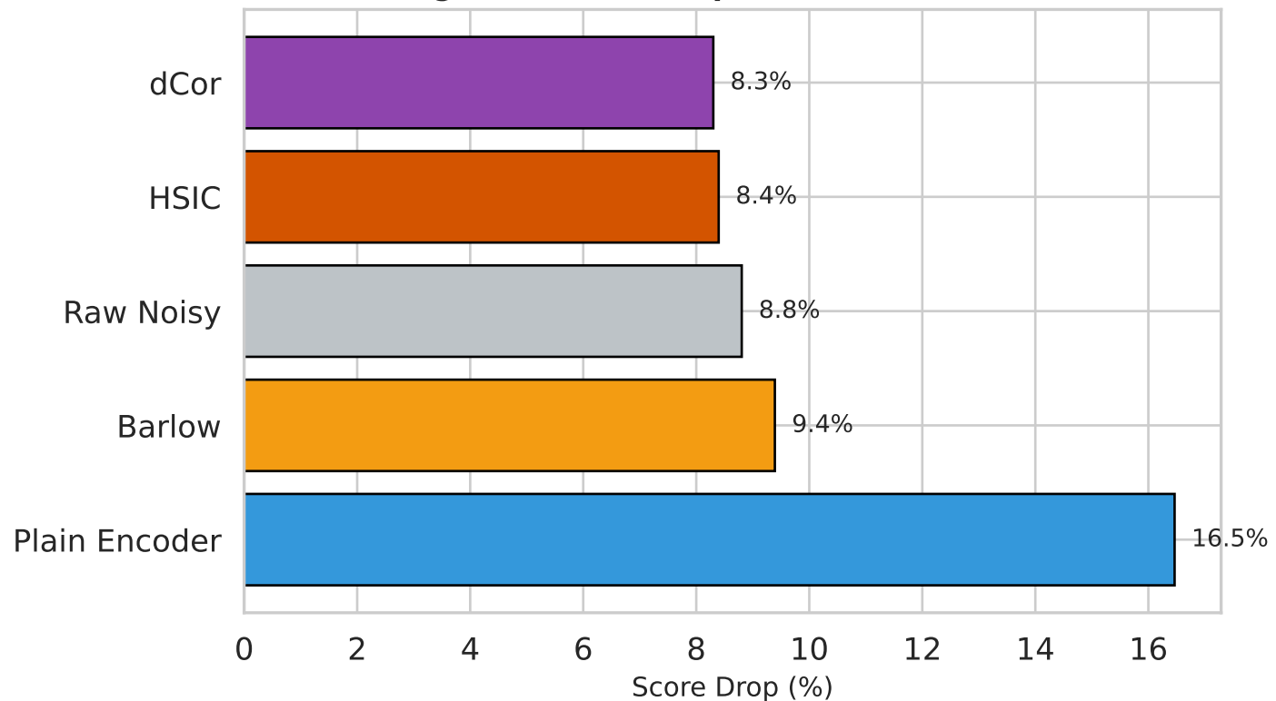
Degradation: % Drop from Scale 0.5 → 2.0
