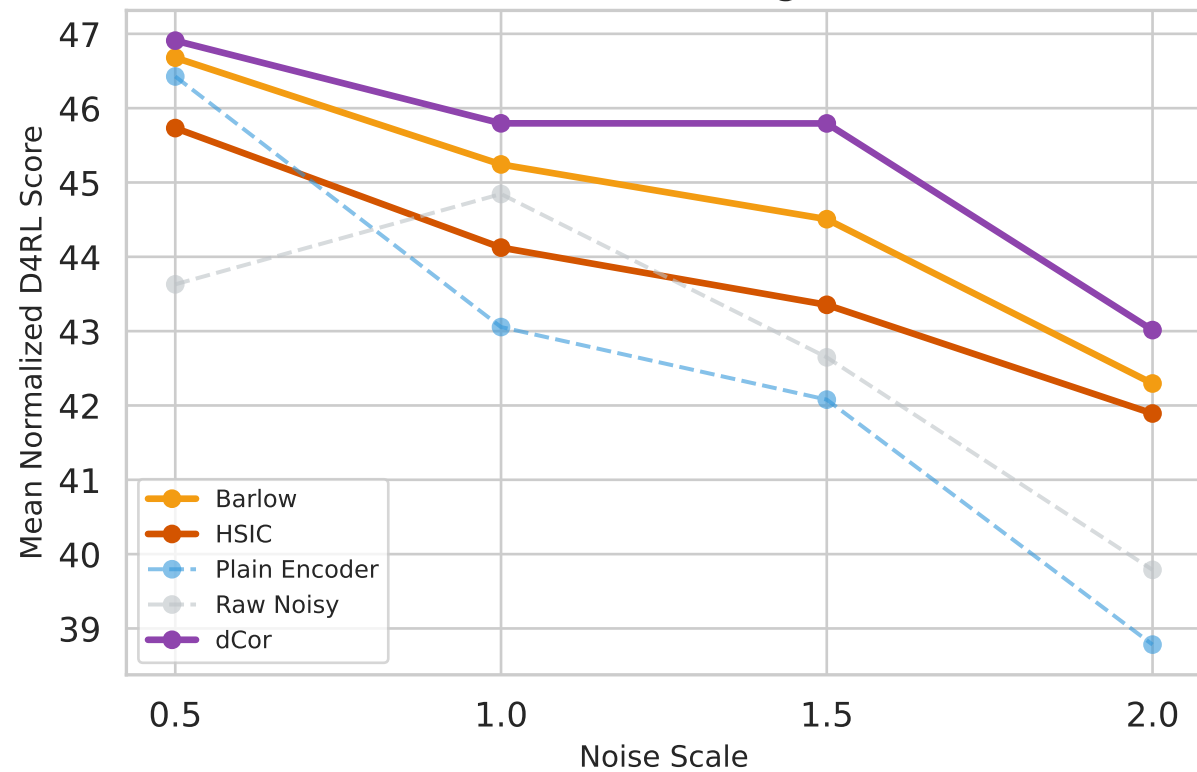
Score vs. Noise Scale (Avg over Dims)
