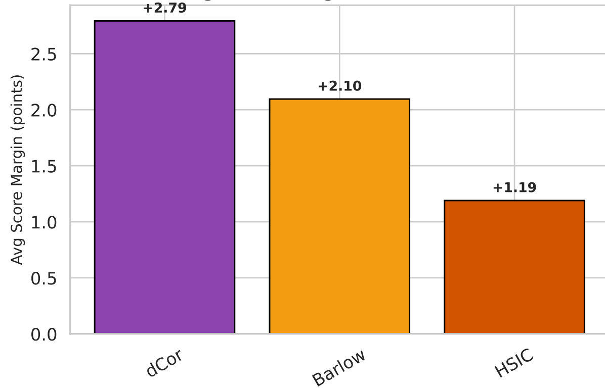
Average Score Margin over Plain Encoder
