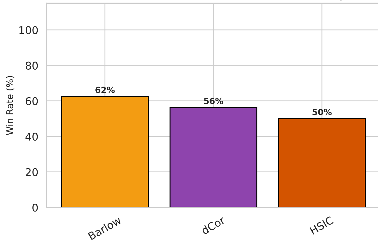
Win Rate vs. Both Baselines (% , out of 16 configs)
