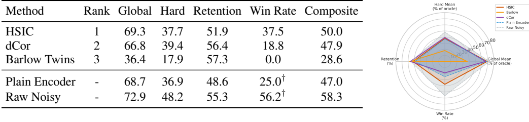
Figure 9: Ant-medium-v2 under nonlinear corruption.
