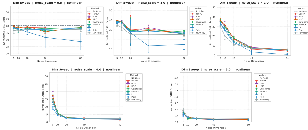
Figure 2: Stage 1 stress-test results on HalfCheetah-medium-v2 under nonlinear corruption.
