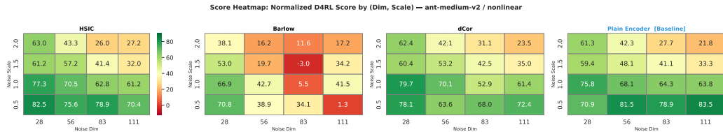
Figure 8: Score heatmap on Ant-medium-v2 under nonlinear corruption.
