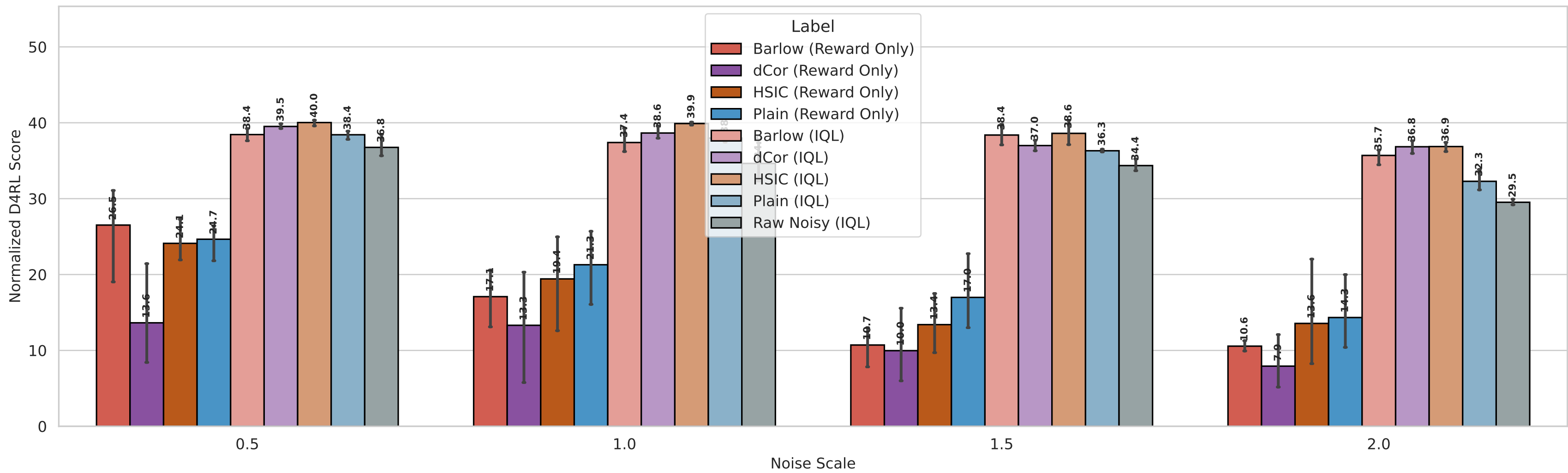
Scale Sweep | noise_dim=4 | ablation_reward_only
