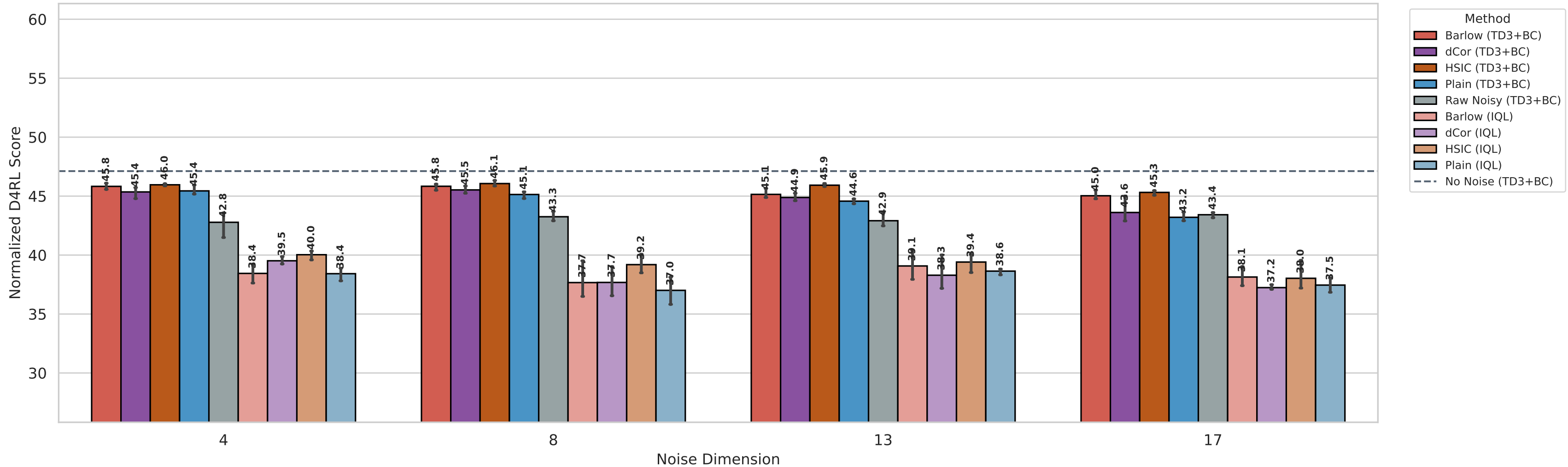
Dim Sweep | noise_scale=0.5 | ablation_td3bc
