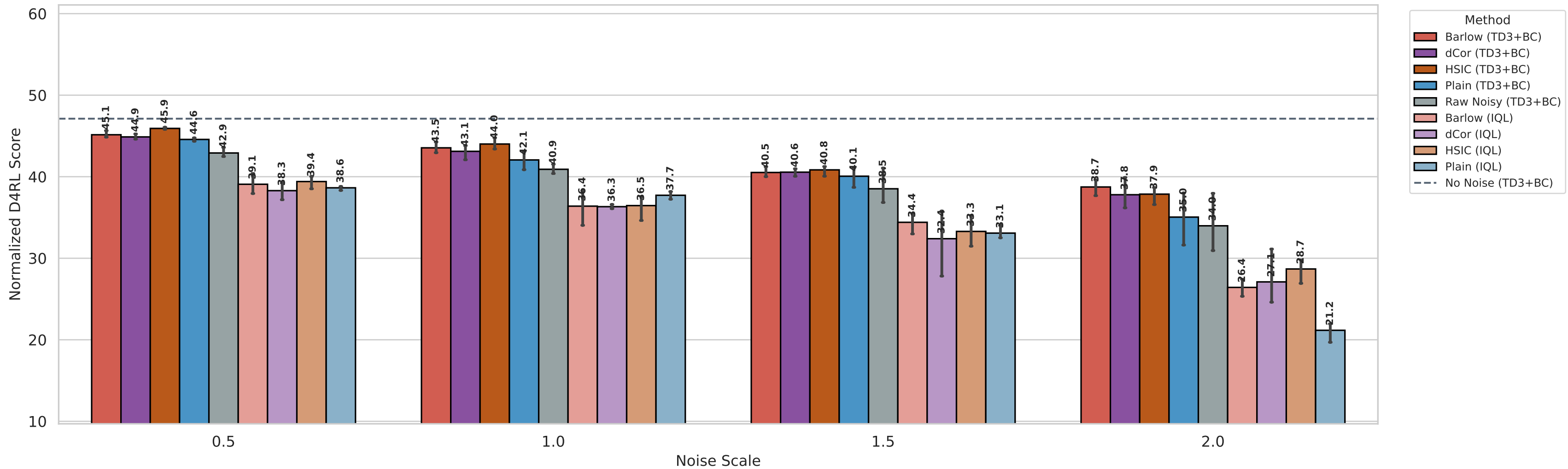
Scale Sweep | noise_dim=13 | ablation_td3bc
