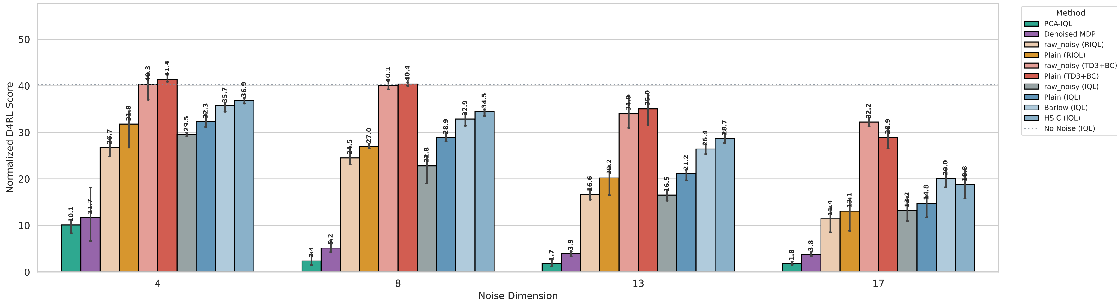
Dim Sweep | noise_scale=2.0 | external methods
