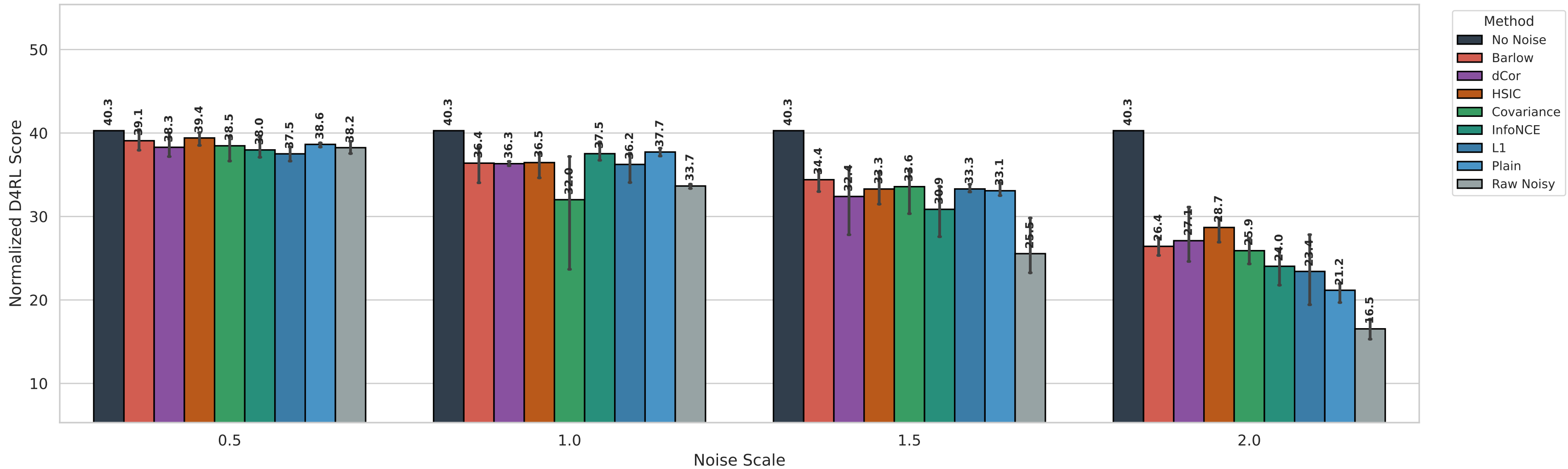
Scale Sweep | noise_dim = 13 | nonlinear
