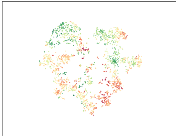
Barlow Twins
