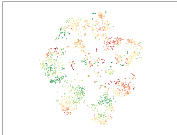
HSIC
