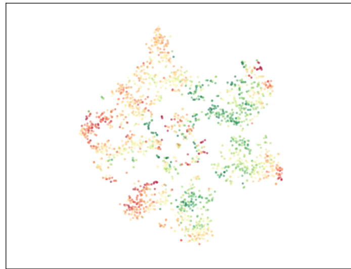
Plain Encoder
