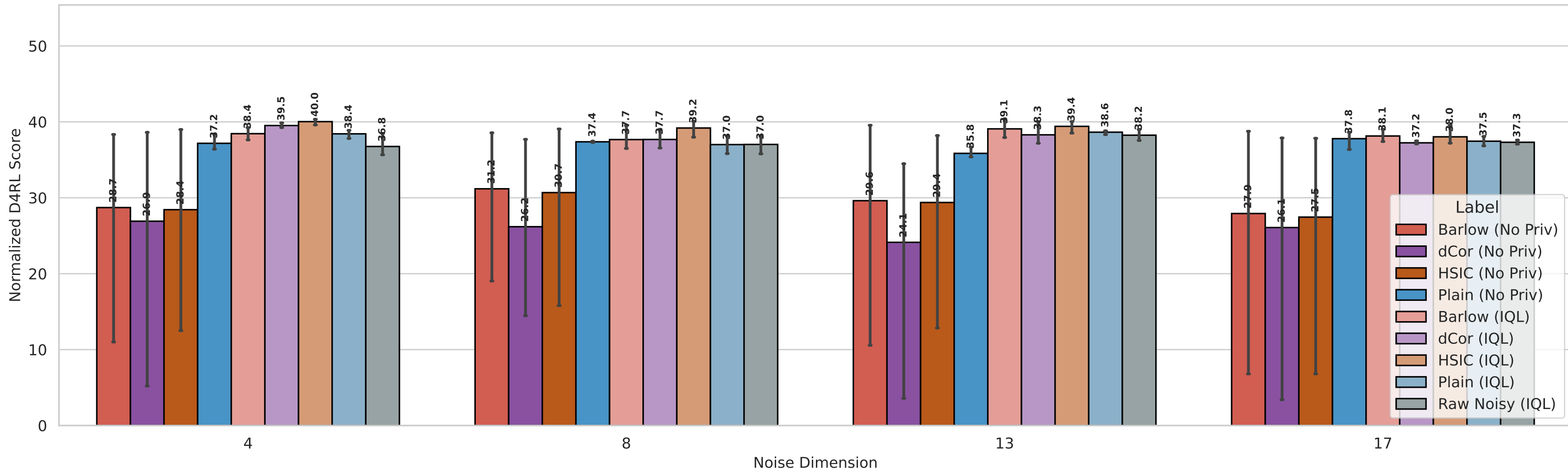
Dim Sweep | noise_scale=0.5 | ablation_noisy_target
