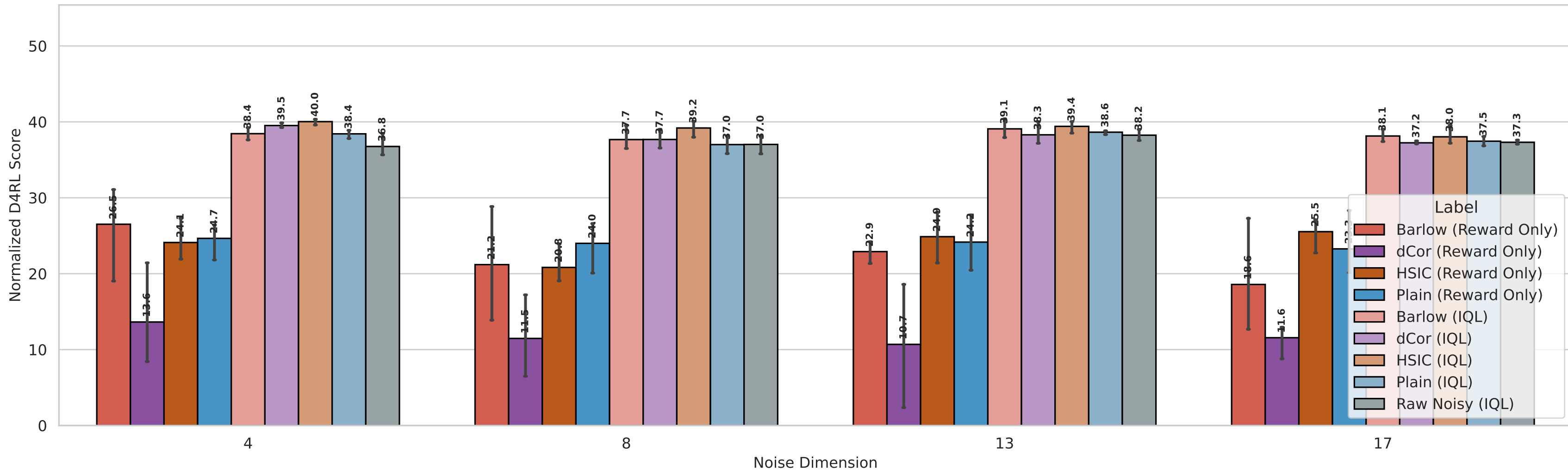
Dim Sweep | noise_scale=0.5 | ablation_reward_only
