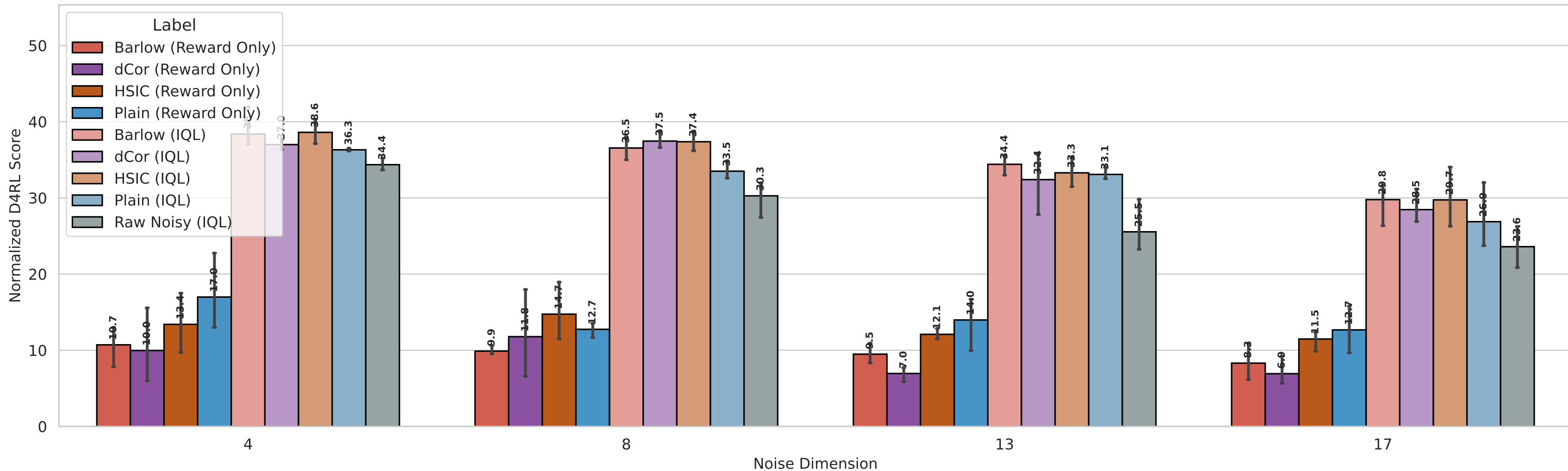
Dim Sweep | noise_scale=1.5 | ablation_reward_only
