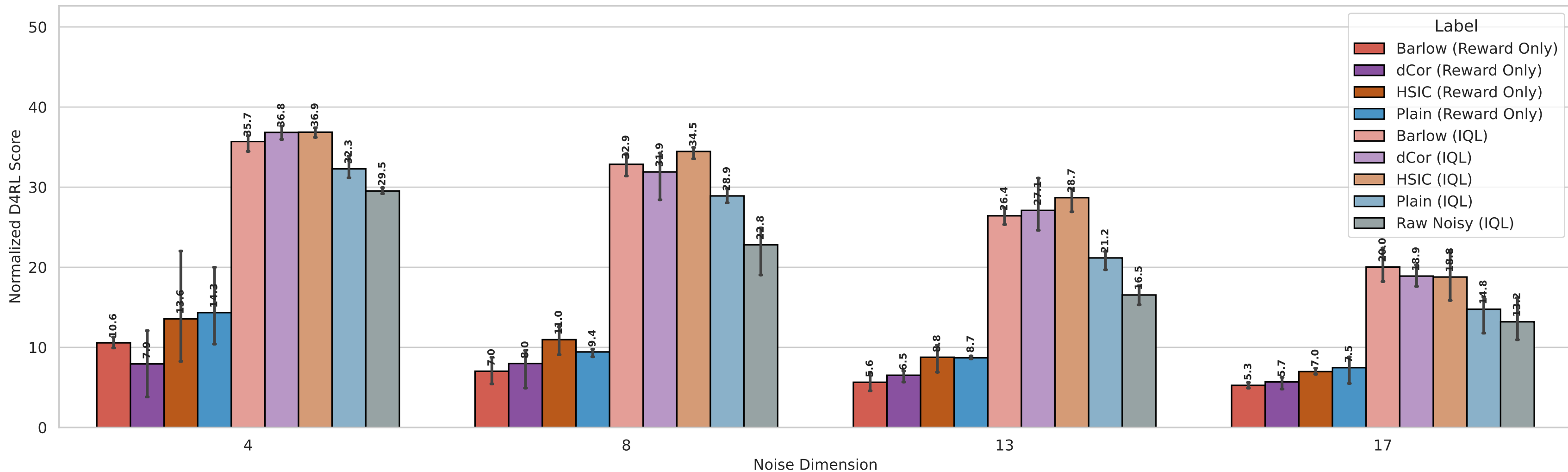
Dim Sweep | noise_scale=2.0 | ablation_reward_only
