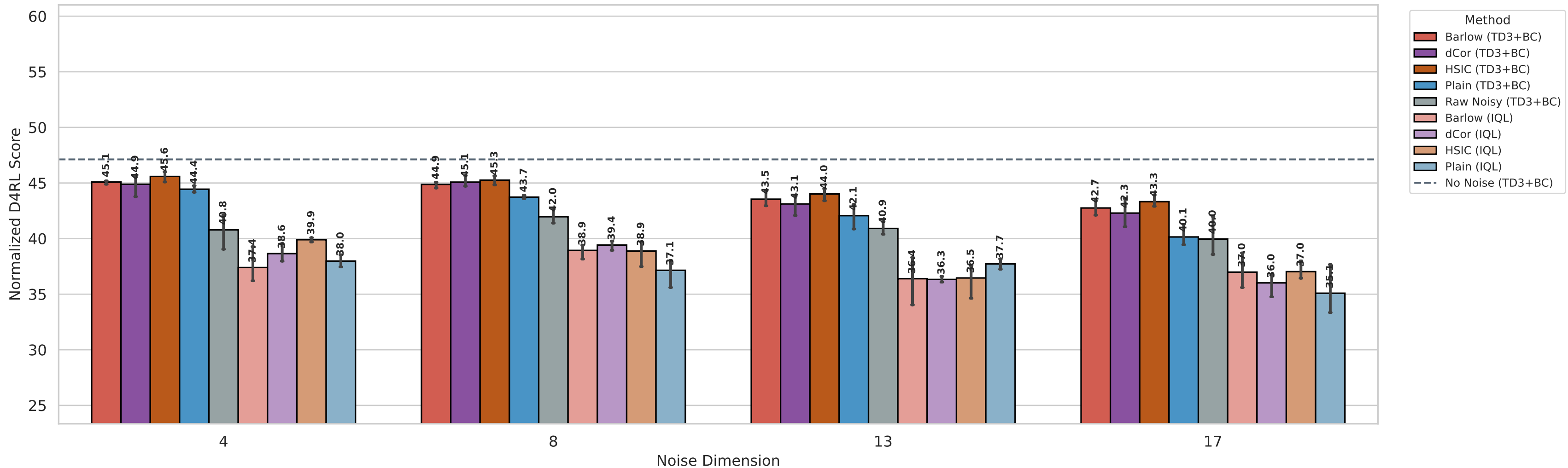
Dim Sweep | noise_scale=1.0 | ablation_td3bc
