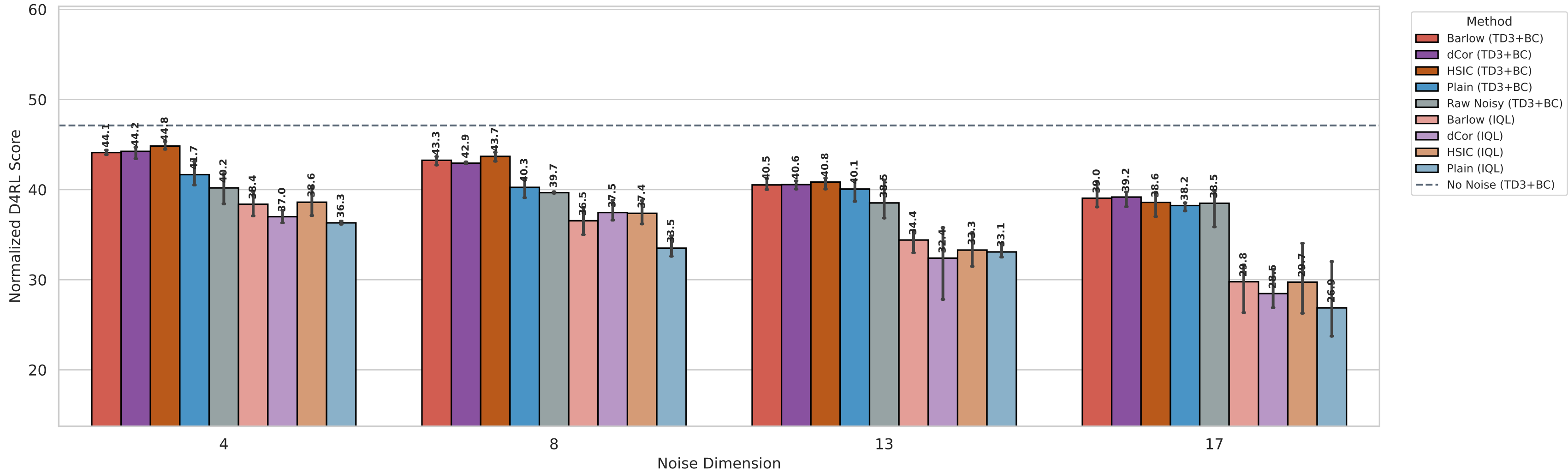
Dim Sweep | noise_scale=1.5 | ablation_td3bc
