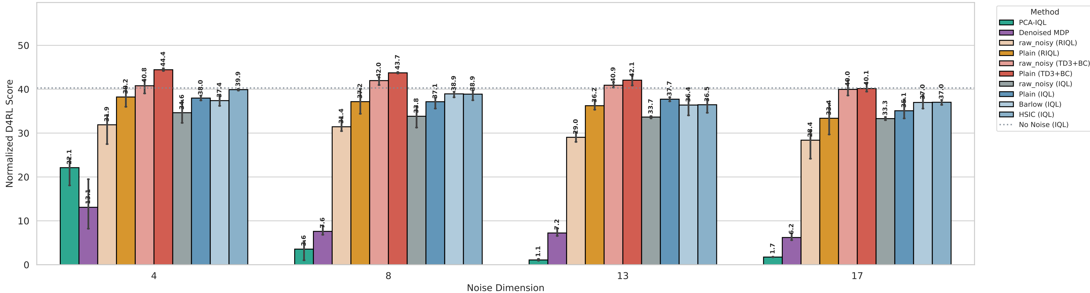
Dim Sweep | noise_scale=1.0 | external methods
