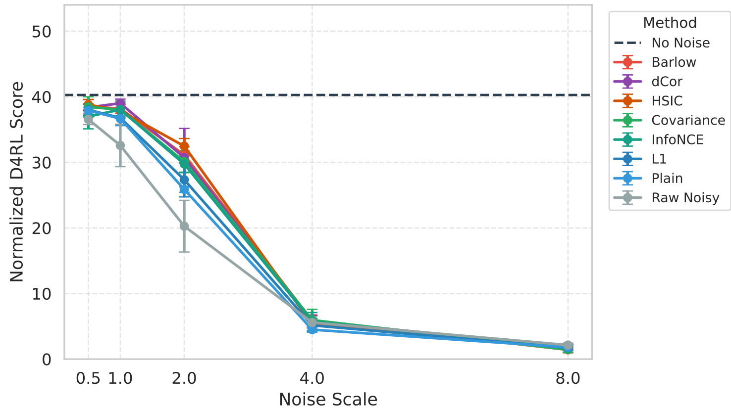
Scale Sweep | noise_dim = 10 | nonlinear
