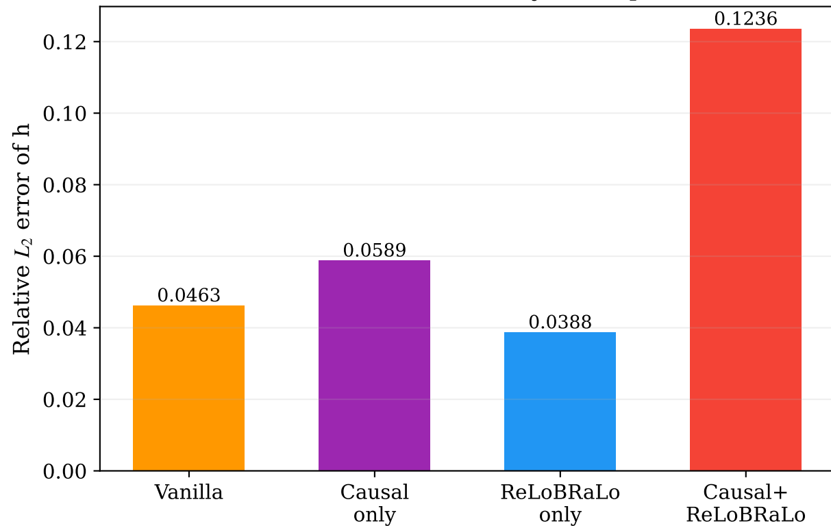
(a) Solution field accuracy (30k epochs)
