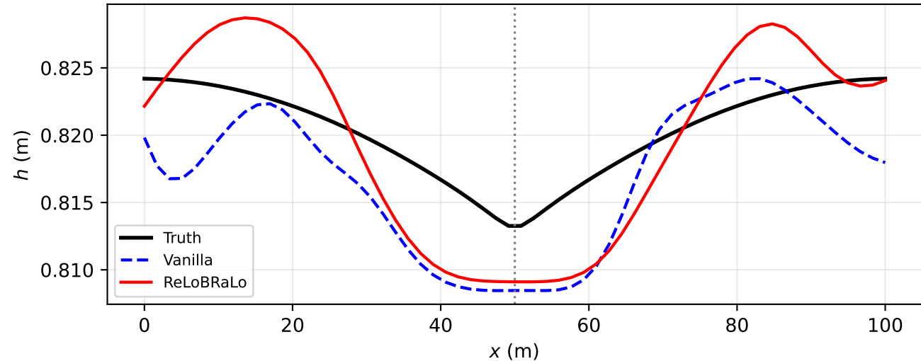
Water depth along y = 50 m at t = 3600 s
