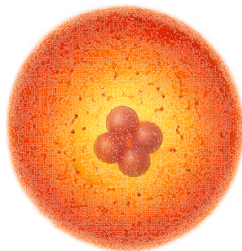
QGP fireball
