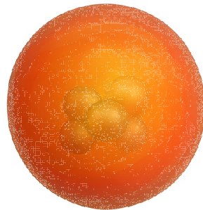
QGP fireball
