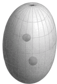
deformed nucleus
