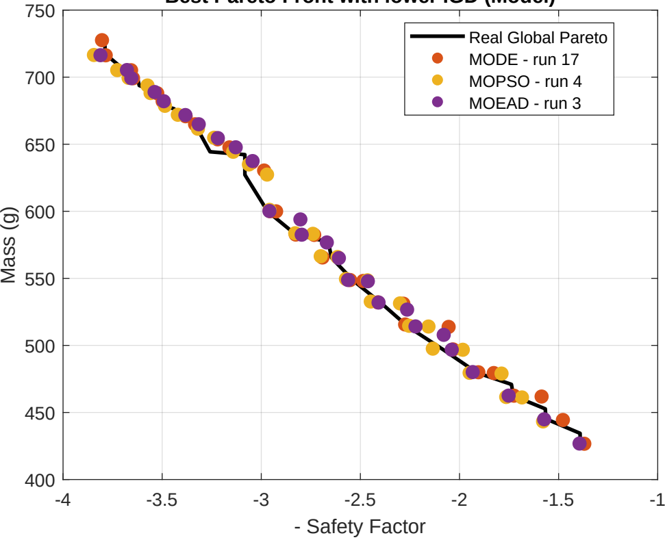
Best Pareto Front with lower IGD (Model)
