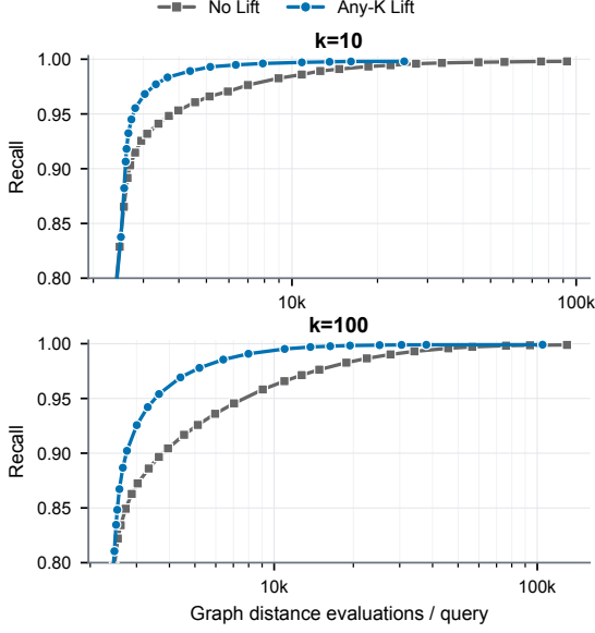
Figure 8: Controlled DEEP1M graph-geometry ablation for k = 10 and 100 . Panels plot recall against graph-distance evaluations per query. No Lift uses the original graph; Lift uses the construction-rank reverse-aware graph. All other components are matched, and precision is 1.0 throughout.
