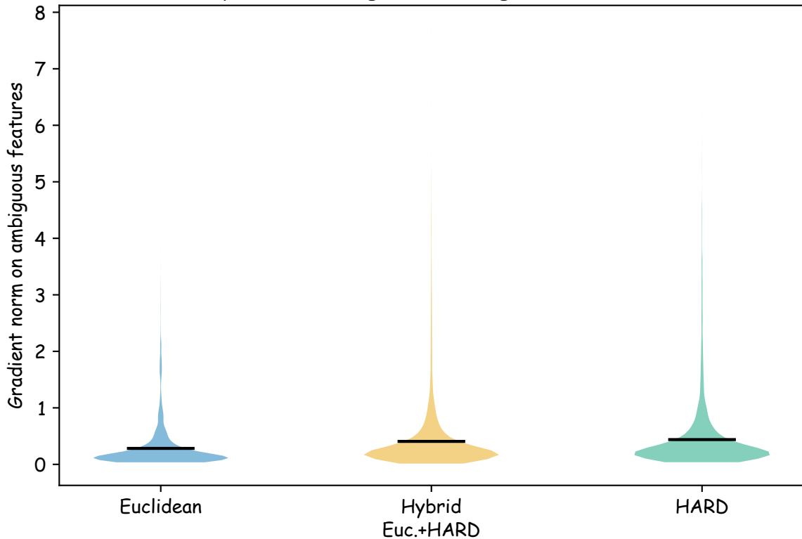
Optimization Signal on Ambiguous Features
