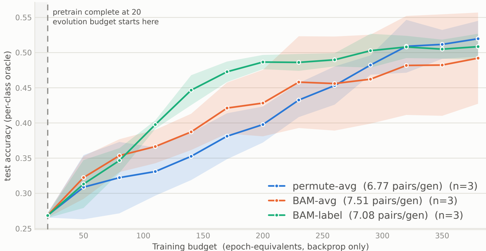
Ablation study on Merging: SESiL (SSL, GS-D-, <Merger>-<Classifier>) at ib=1.5
