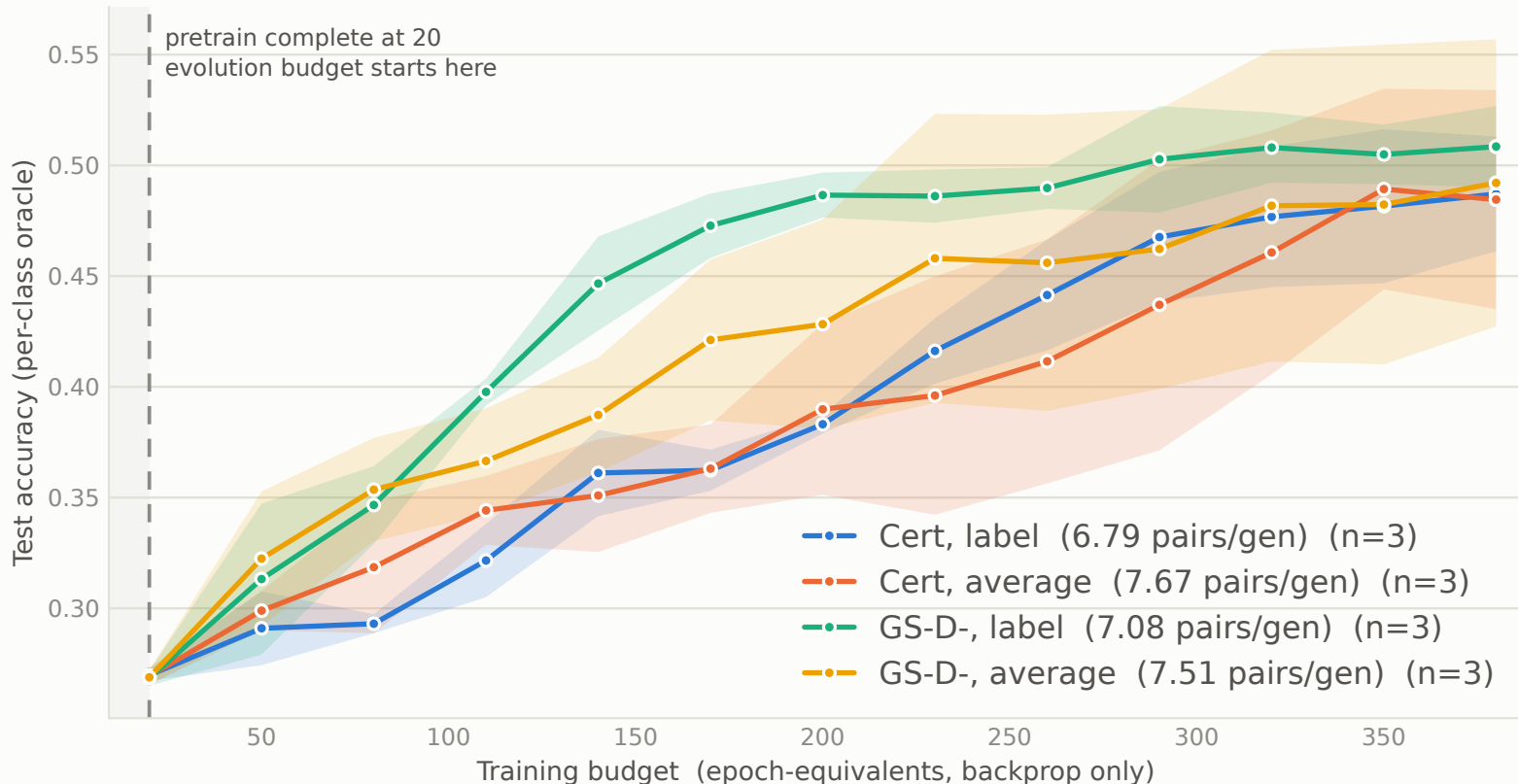
Ablation Study on Mating: SESiL-GS (SSL, <Selector>, BAM-<Classifier>)
