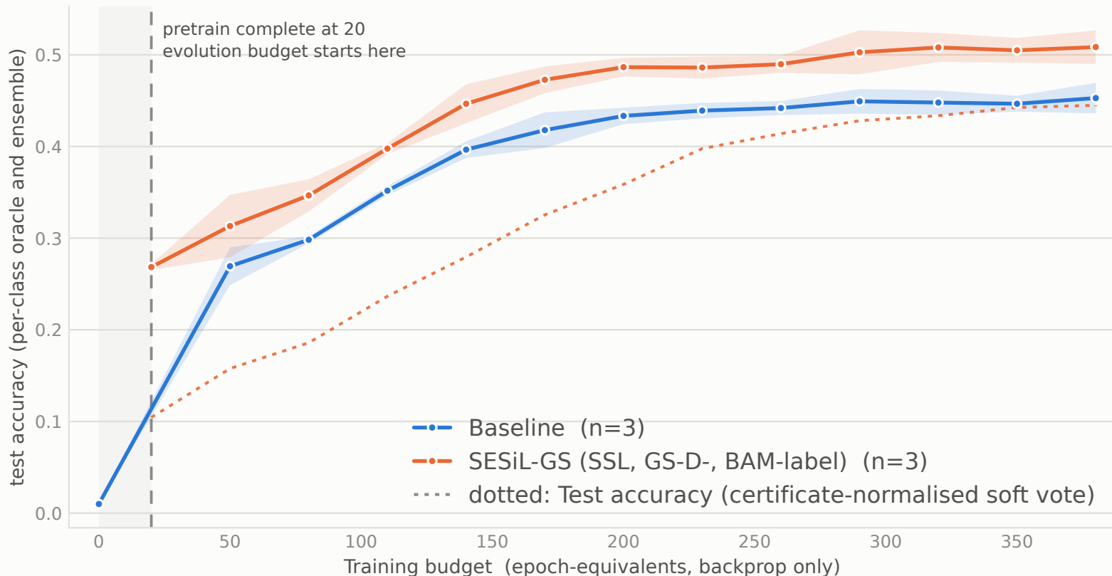
SESiL-GS vs Baseline on CIFAR-100: per-class oracle and ensemble decision
