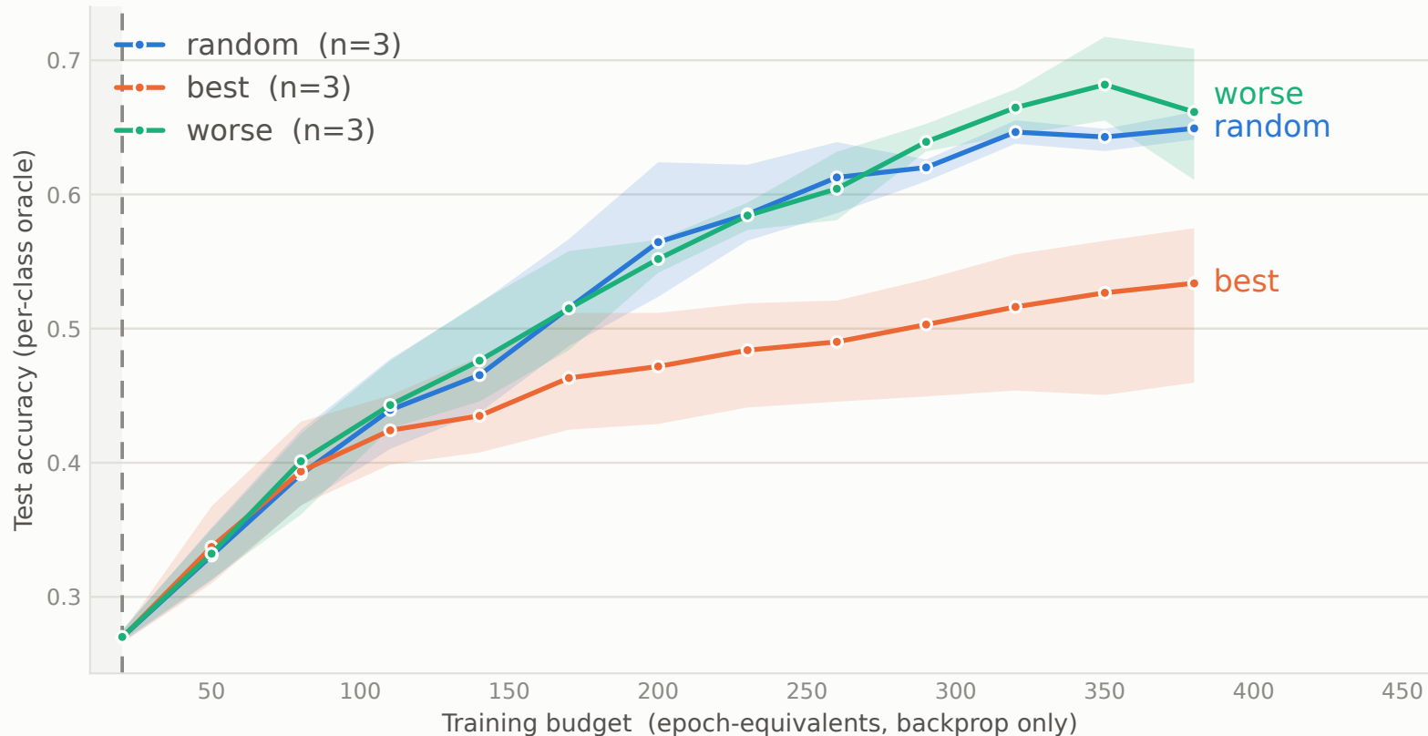
SESiL (ssl, cert, permute-avg) on mutation modes in {random, best, worse}
