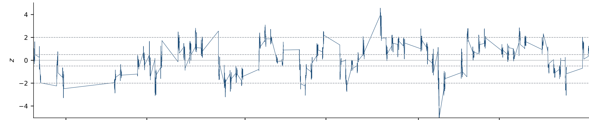
Kalman z-score
