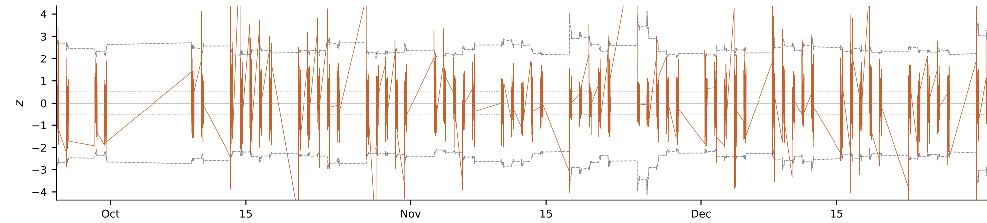
Kalman z-score
