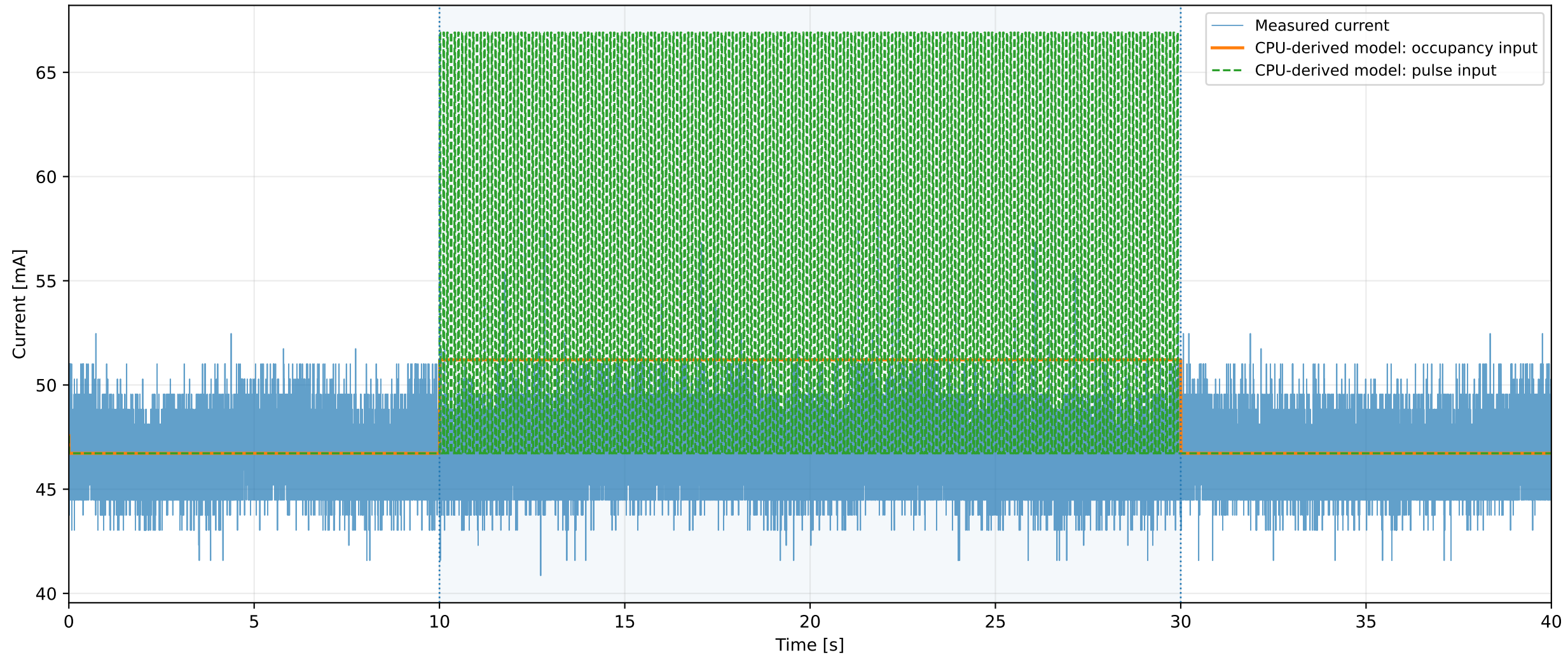
UART TX-only workload: measured current vs CPU-derived model UART 256 B / 100 ms, representative run
