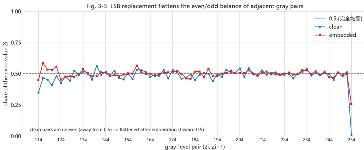
Figure 7: Fig. 3-3 even/odd counts of adjacent gray pairs: clean vs embedded
