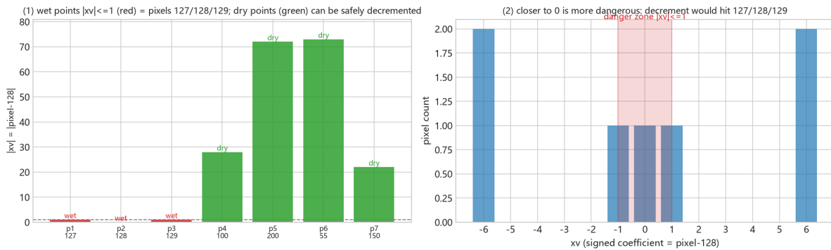
Figure 12: Fig. 5-1 wet/dry partition
