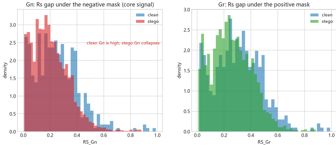
Figure 24: Fig. 8-1 RS feature distributions
