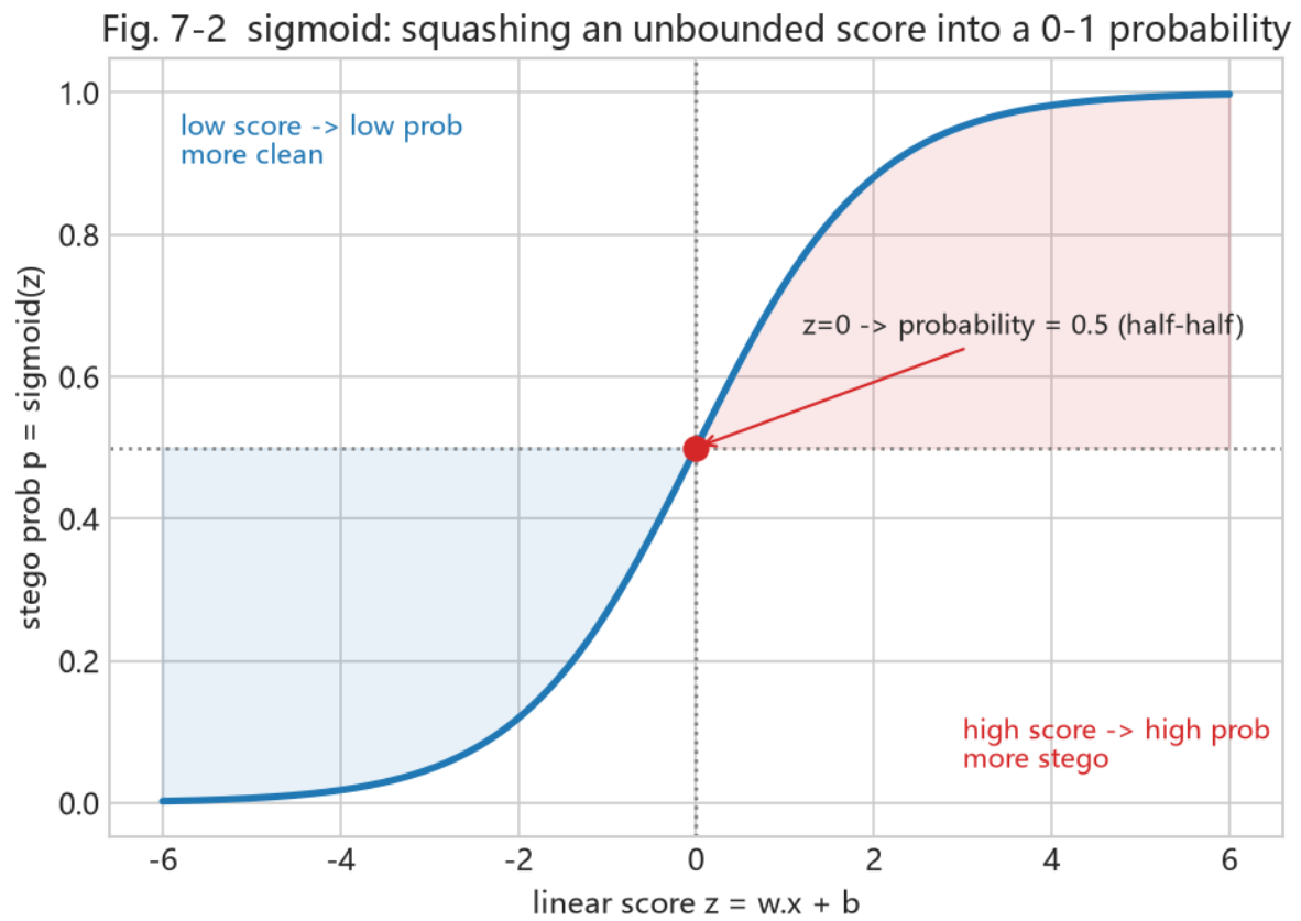
Figure 17: Fig. 7-2 sigmoid
