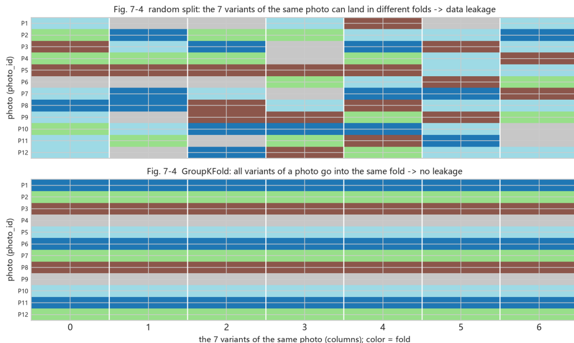
Figure 19: Fig. 7-4 GroupKFold
