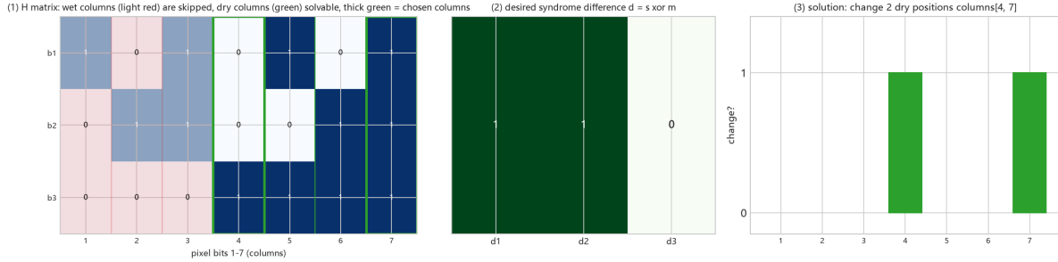
Figure 13: Fig. 5-2 wet paper solving
