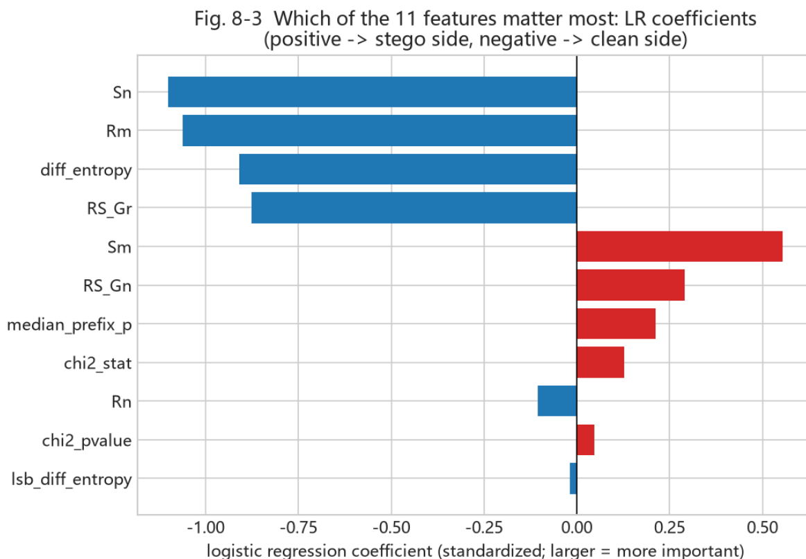
Figure 27: Fig. 8-3 feature importance
