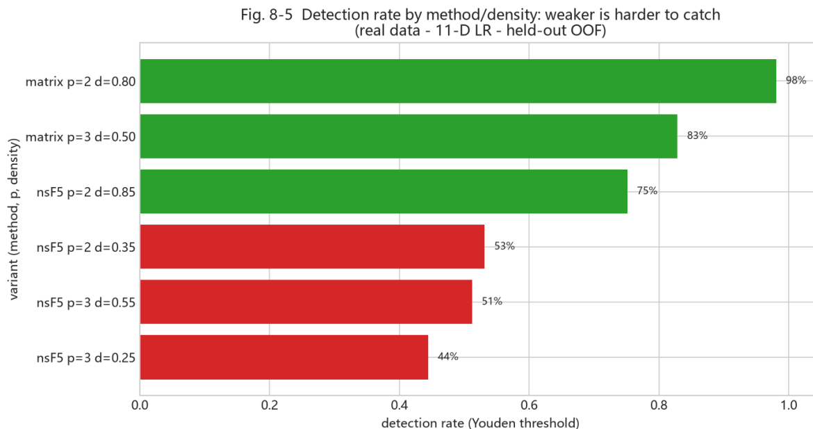
Figure 28: Fig. 8-5 per-density detection
