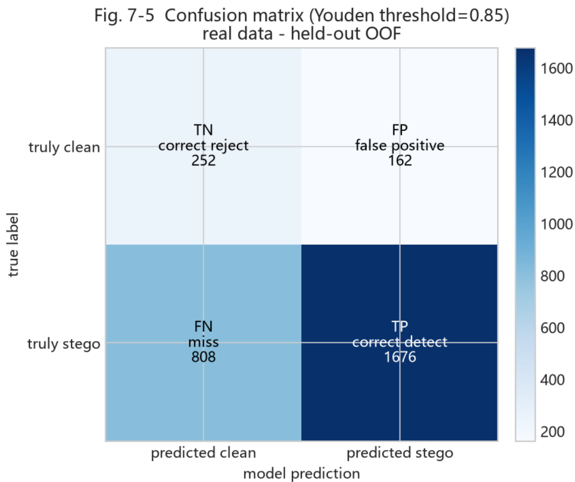
Figure 20: Fig. 7-5 confusion matrix
