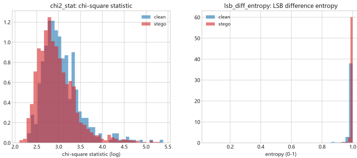
Figure 25: Fig. 8-2 chi-square/entropy feature distributions
