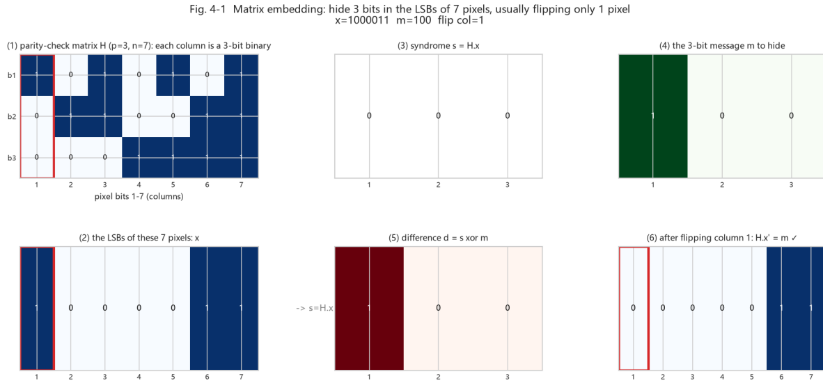
Figure 9: Fig. 4-1 matrix-coding syndrome schematic
