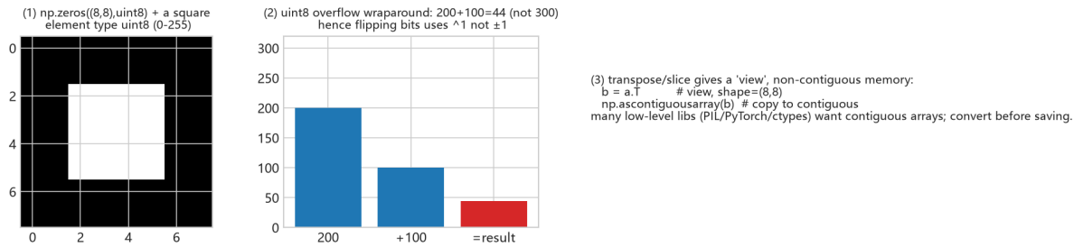
Figure 4: Fig. 2-2 dtype and memory layout
