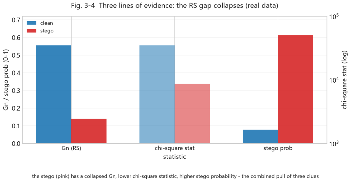
Figure 8: Fig. 3-4 three lines of evidence: RS gap / chi-square statistic / stego probability
