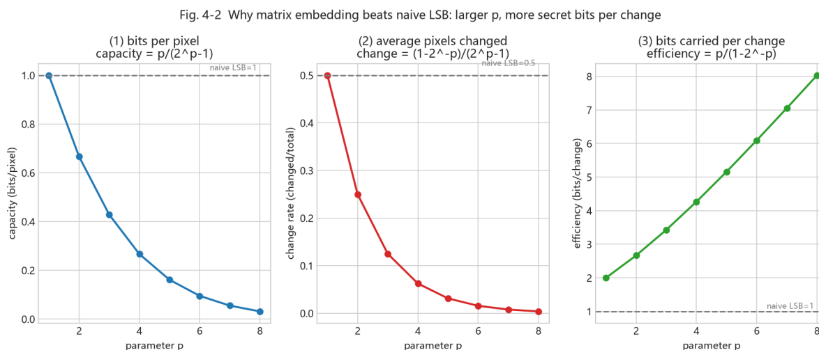
Figure 10: Fig. 4-2 embedding efficiency
