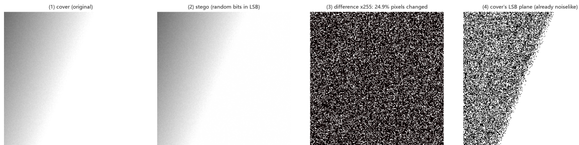
Figure 5: Fig. 3-1 cover vs stego vs amplified diff
