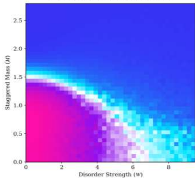
Kane-Mele Phase Diagram ( t_R=0.0 )
