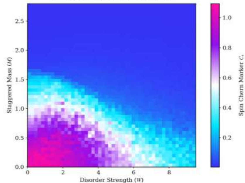
Kane-Mele Phase Diagram ( t_R=0.6 )
