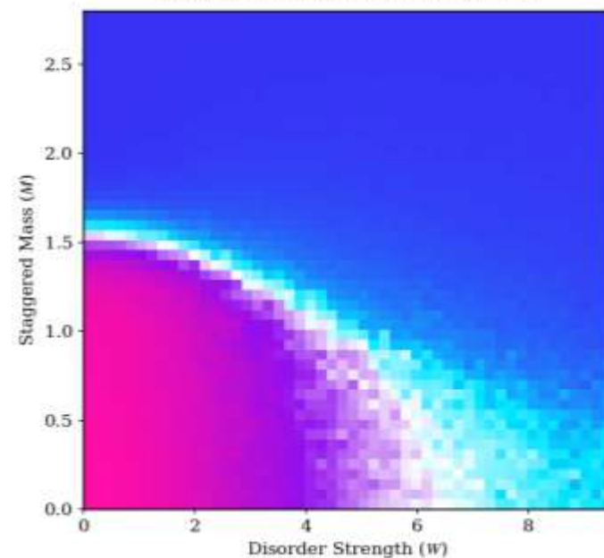
Kane-Mele Phase Diagram ( t_R=0.2 )
