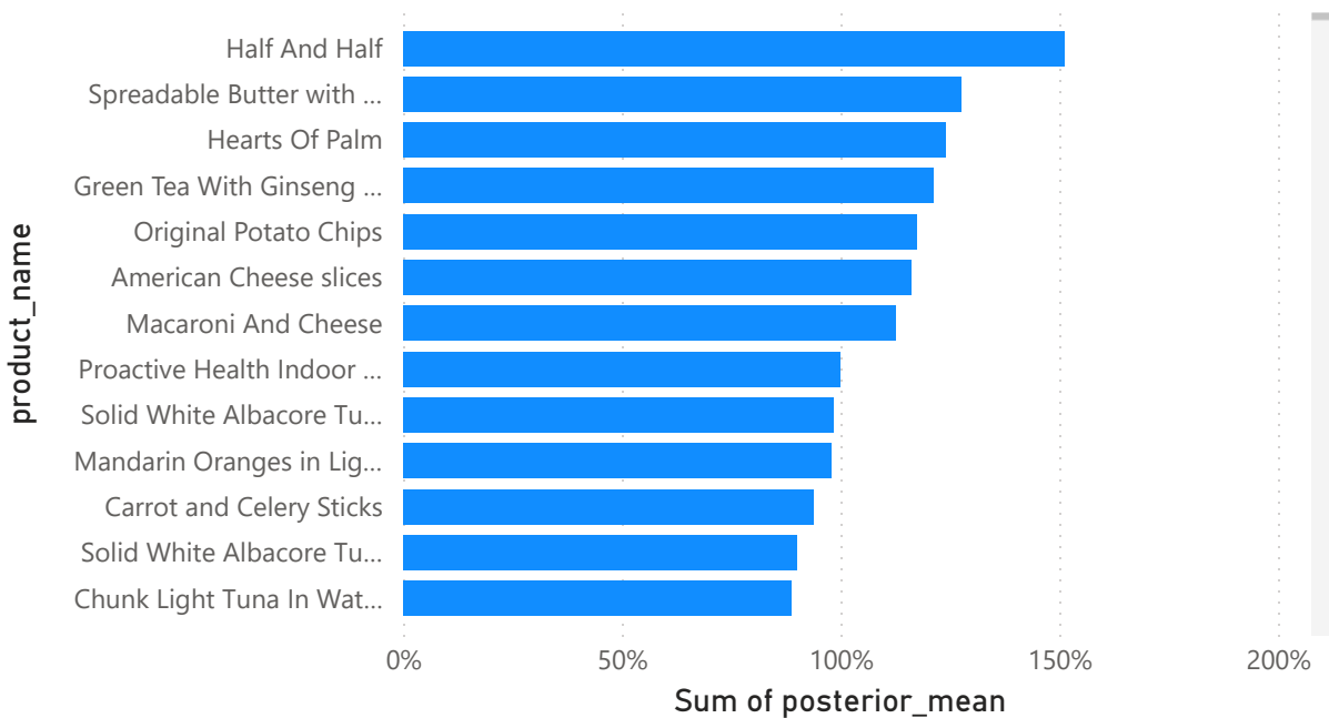
Sum of posterior_mean by product_name
