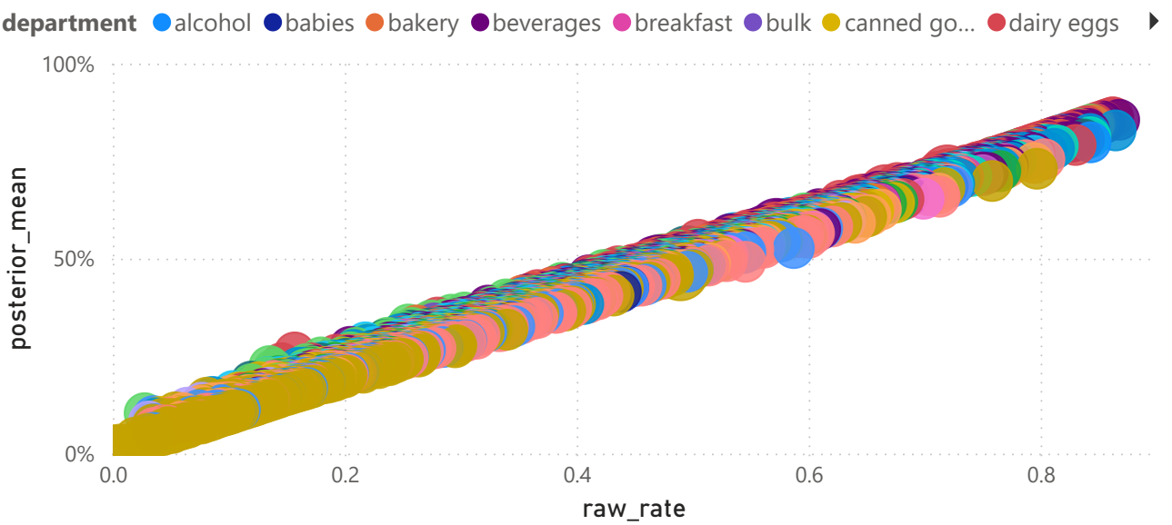
Count of times_ordered by department, raw_rate and posterior_mean
