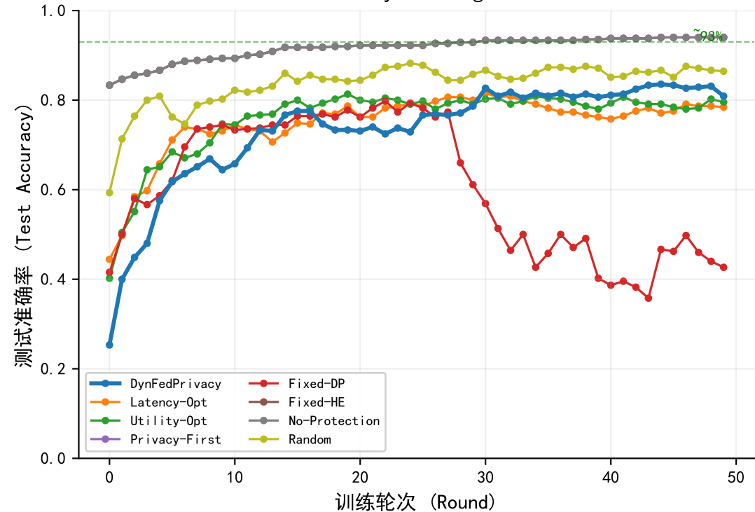
(a) 精度收敛曲线 Accuracy Convergence
