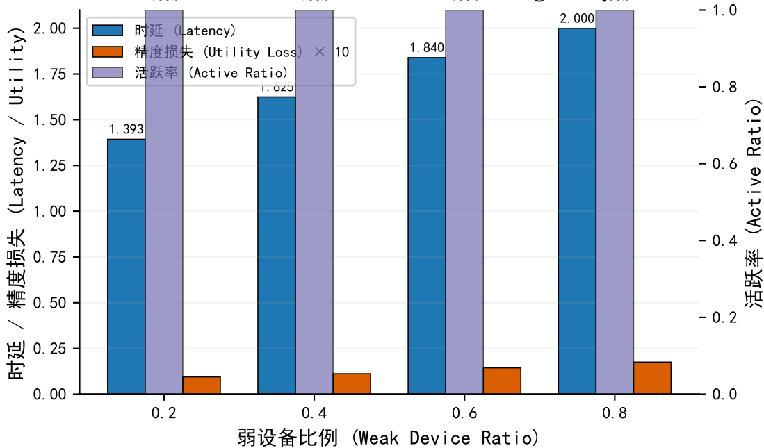
DynFedPrivacy: 资源异构性下的综合表现 Performance under Resource Heterogeneity
