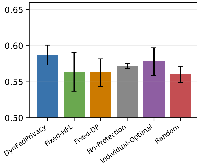
Avg-last-10 accuracy
