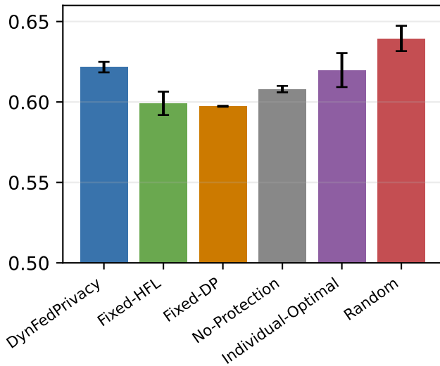
Best accuracy
