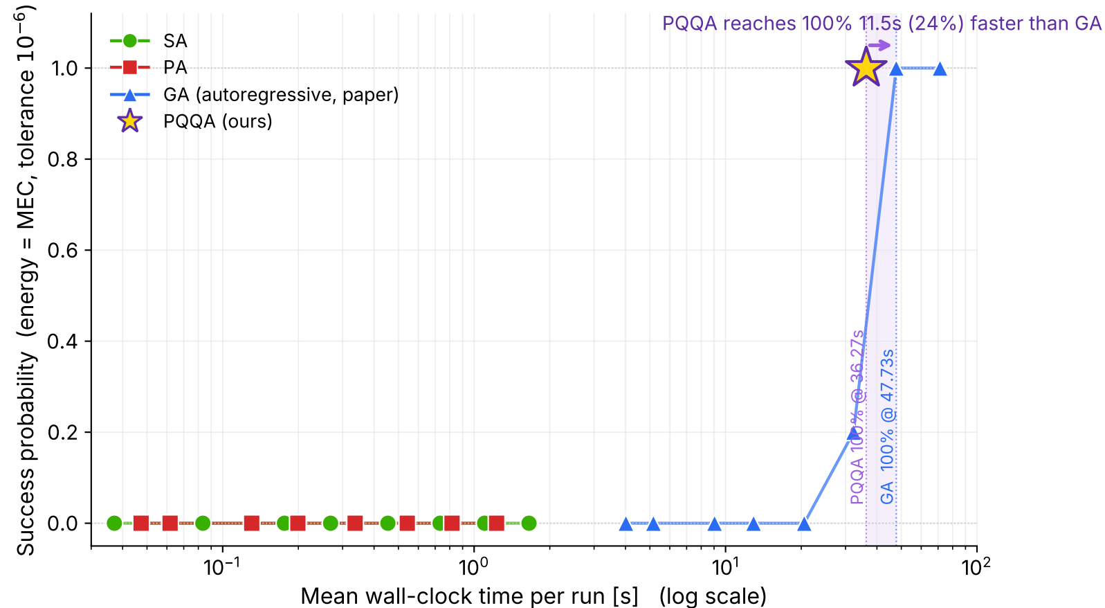
L=10 hard instance (seed 310411727) — Success vs wall-clock time
