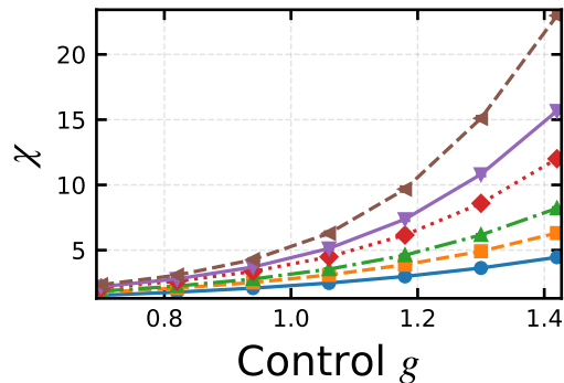
Susceptibility \chi
