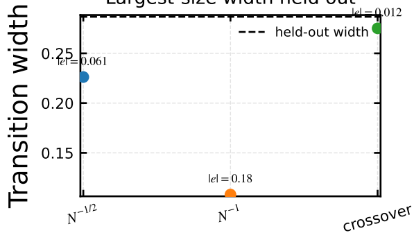
Largest-size width held out
