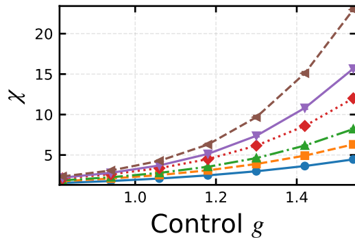
Susceptibility \chi
