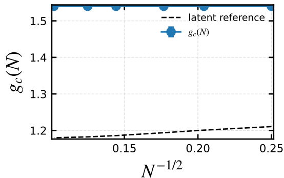
Pseudocritical drift
