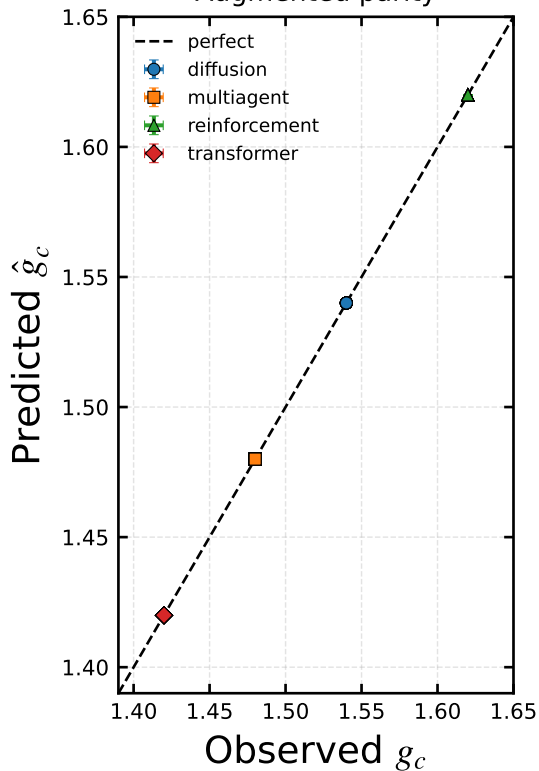
Augmented parity
