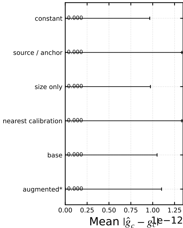
Holdout benchmark
