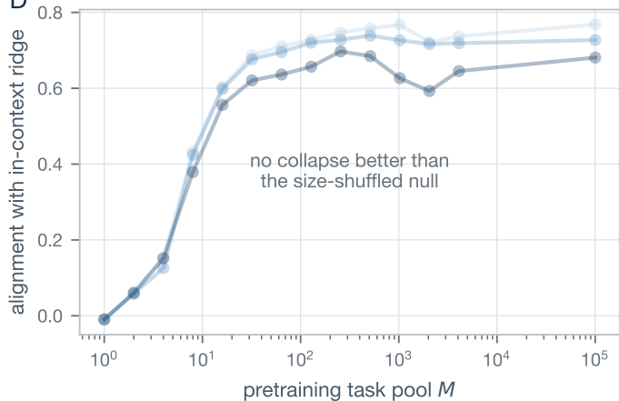
D Finite-size collapse
