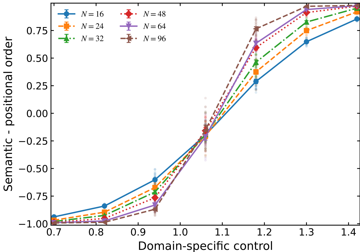
Transformer: finite-size holdout
