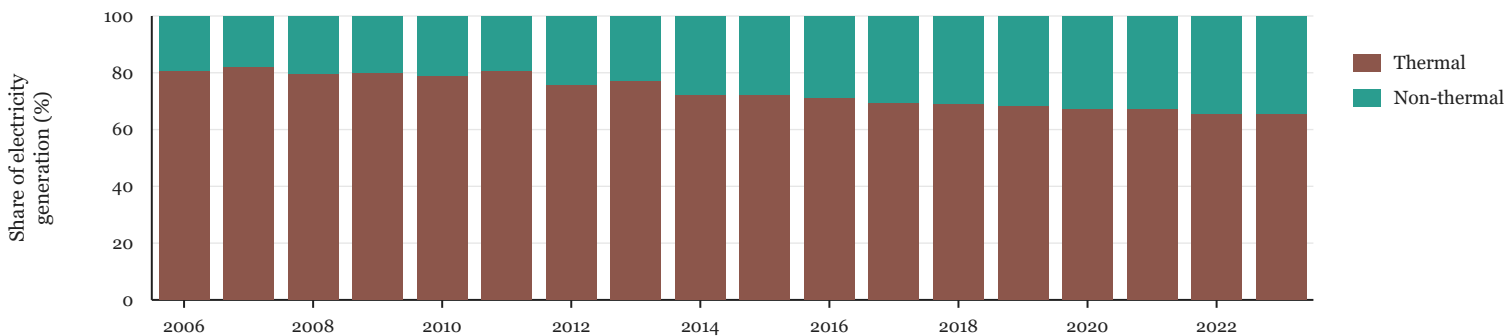
(c) Electricity-generation composition
