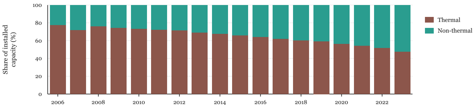
(b) Installed power-capacity composition
