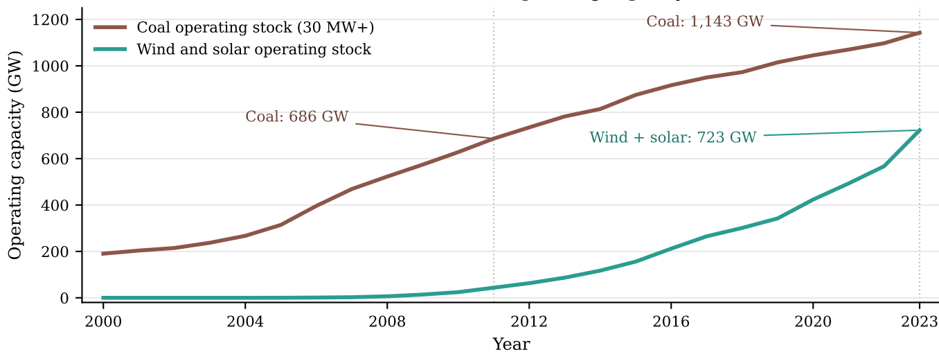
(b) Reconstructed operating capacity
